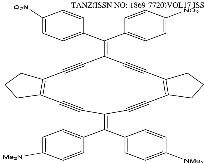
Fig.2 Proaromatic Compound
